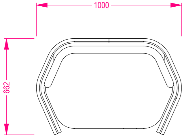
Plan Elevation
